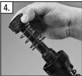
4. Unscrew the piston guide nut counterclockwise until it comes off.
