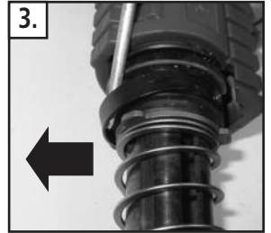
3. Remove piston stopper clip
